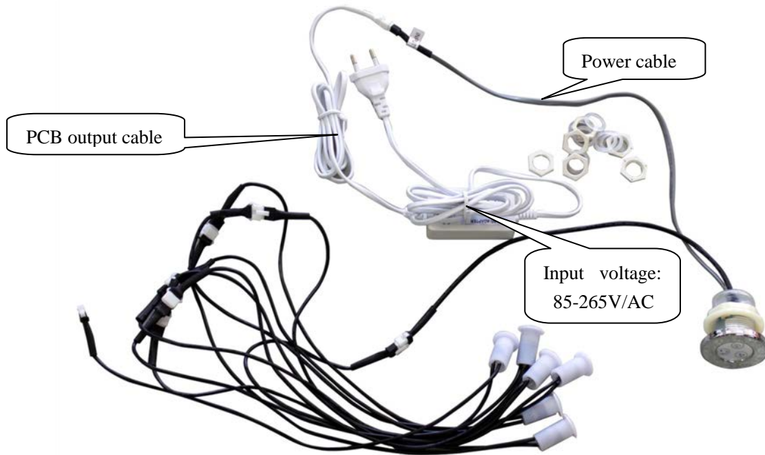
Picture 1: Coupling of accessories
